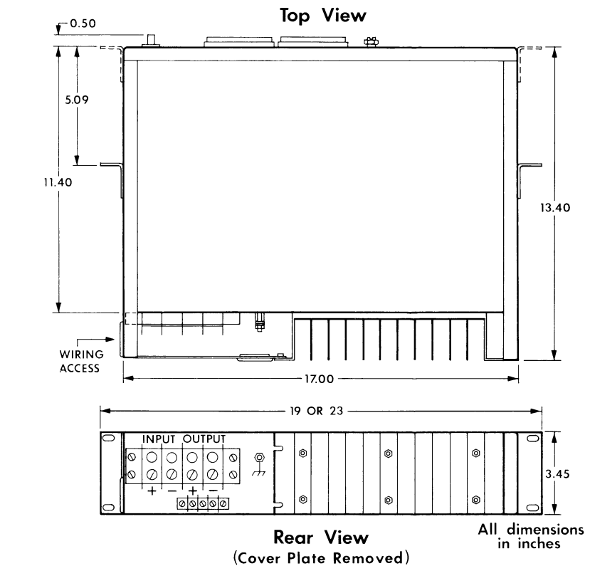
Fig. 1 Model 1605 overall dimensions
