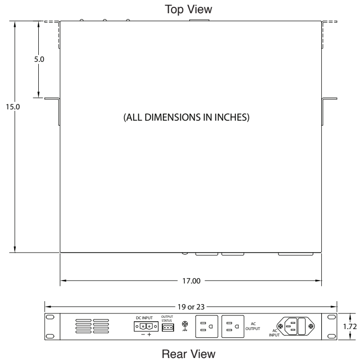
Fig. 1 Overall dimensions. Inverter shown is U or L version.
